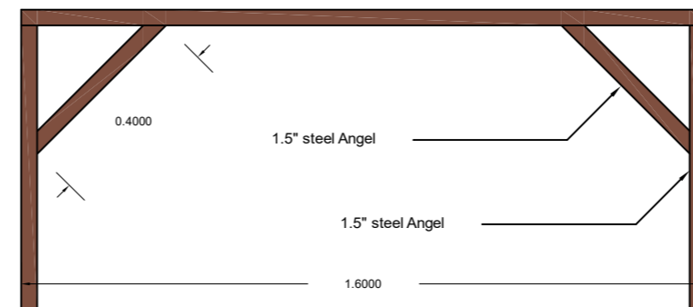
Desk Typical Section at (X-X)
