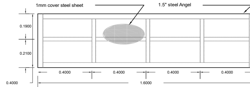
Desk Typical Plan At Top
