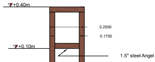
Seat Typical Section at (B-B)
