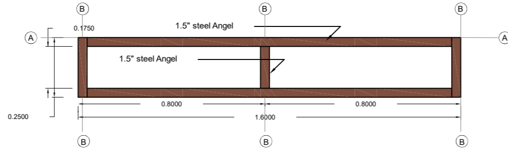
Seat Typical Plan without Steel Plate
