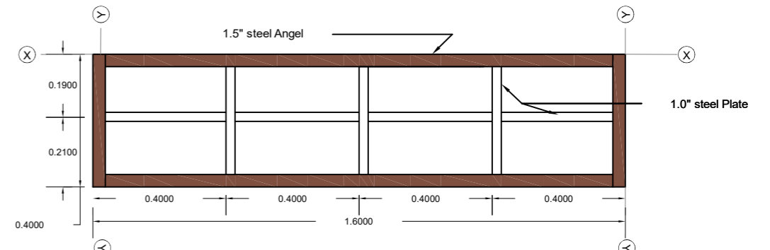
Desk Typical Plan below steel sheet
